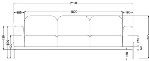
3 SEATER DX-VLR-03-TS 2190(L) X 765(W) X 420(SH) X 780(H)
