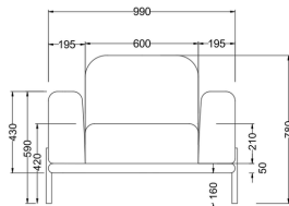
1 SEATER DX-VLR-01-SS 990(L) X 765(W) X 420(SH) X 780(H)
