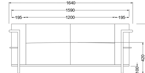
2.5 SEATER DX-HCT-02-DS 1640(L) X 820(W) X 420(SH) X 670(H)
