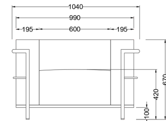
1.5 SEATER DX-HCT-01-SS 1040(L) X 820(W) X 420(SH) X 670(H)
