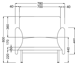
1 SEATER DX-CPT-01-SS 780(L) X 780(W) X 440(SH) X 800(H)
