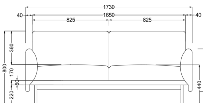
2.5 SEATER DX-CPT-2.5-DS 1730(L) X 780(W) X 440(SH) X 800(H)
