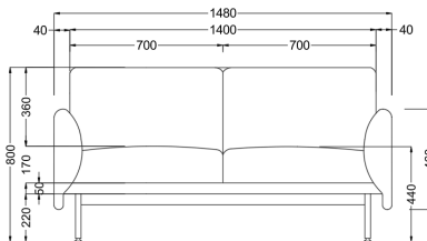
2 SEATER DX-CPT-02-DS 1480(L) X 780(W) X 440(SH) X 800(H)
