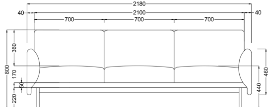
3 SEATER DX-CPT-03-TS 2180(L) X 780(W) X 440(SH) X 800(H)
