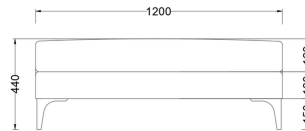
2.5 OTTOMAN DX-CMD-02S-BS 1200(L) X 725(W) X 440(H)
