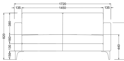
2.5 SEATER DX-CMD-2.5-DS 1720(L) X 860(W) X 440(SH) X 820(H)
