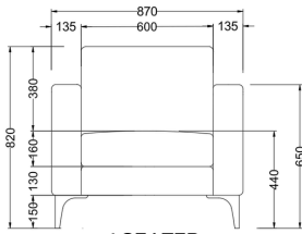
1 SEATER DX-CMD-01-SS 870(L) X 860(W) X 440(SH) X 820(H)
