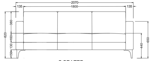
3 SEATER DX-CMD-03-TS 2070(L) X 860(W) X 440(SH) X 820(H)
