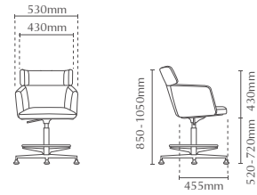
PT6631L-15RH Presidential medium back - AB15 4 pronged aluminium base with stud, chrome high gas lift & footrest ring - MH101 ball motion mechanism
