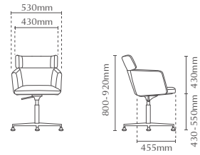
PT6631L-15 Presidential medium back - AB15 4 pronged aluminium base with stud & chrome gas lift - MH101 ball motion mechanism
