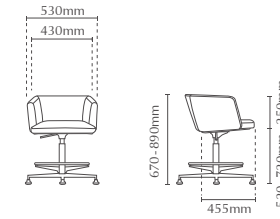
PT6632L-15RH Executive low back - AB15 4 pronged aluminium base with stud, chrome high gas lift & footrest ring - MH101 ball motion mechanism
